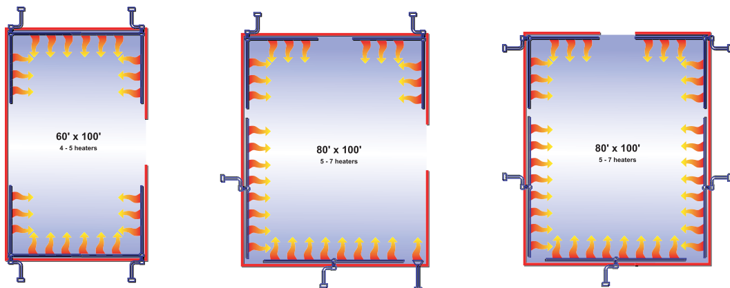
Sample Premier 170 distribution installations.
