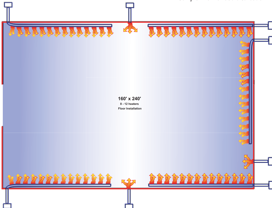
Sample Premier 350 distribution installations.
